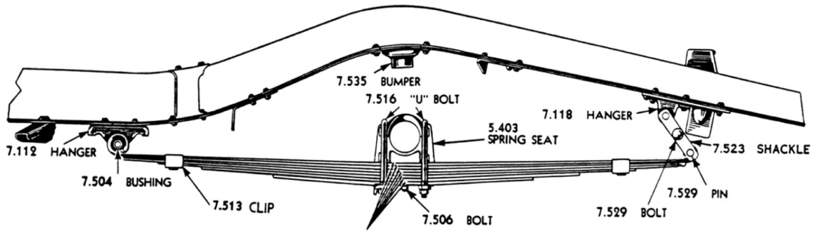
REAR SPRING AND PARTS
