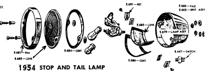
1954 STOP AND TAIL LAMP
