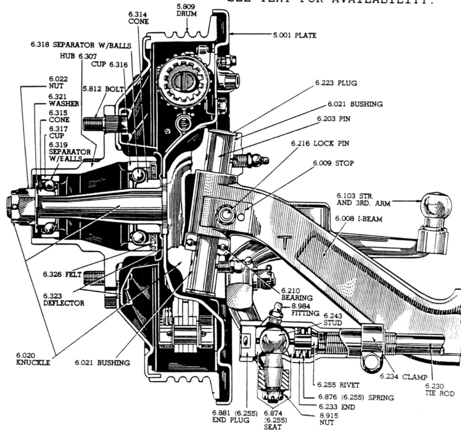
FRONT AXLE—CONVENTIONAL TRUCK (EXC. HVY. DUTY)
