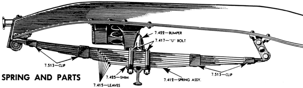
REAR SPRING AND PARTS
