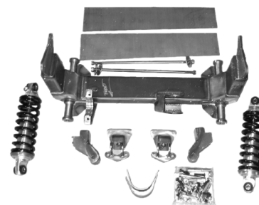
IFS kit shown with optional coil overs
