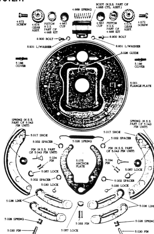
HYDRAULIC BRAKE PARTS—FRONT
